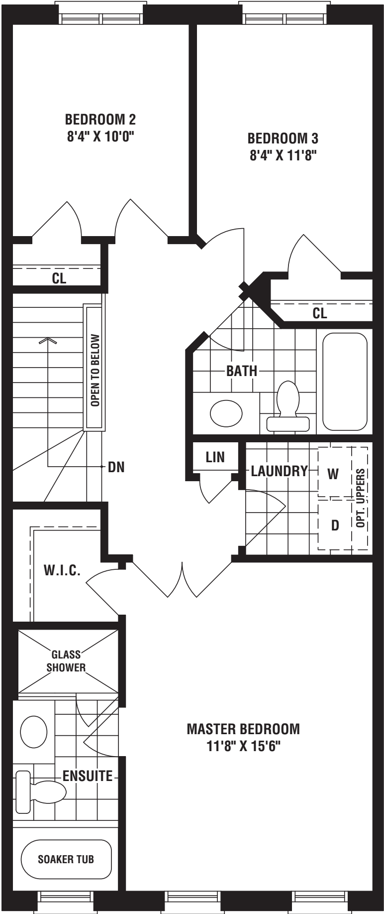
SECOND FLOOR ELEV. 'A' & 'B'
