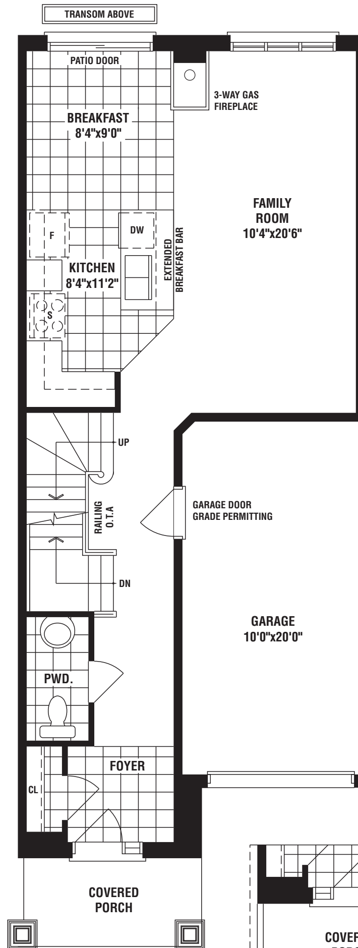
GROUND FLOOR PLAN EL. 'A'
