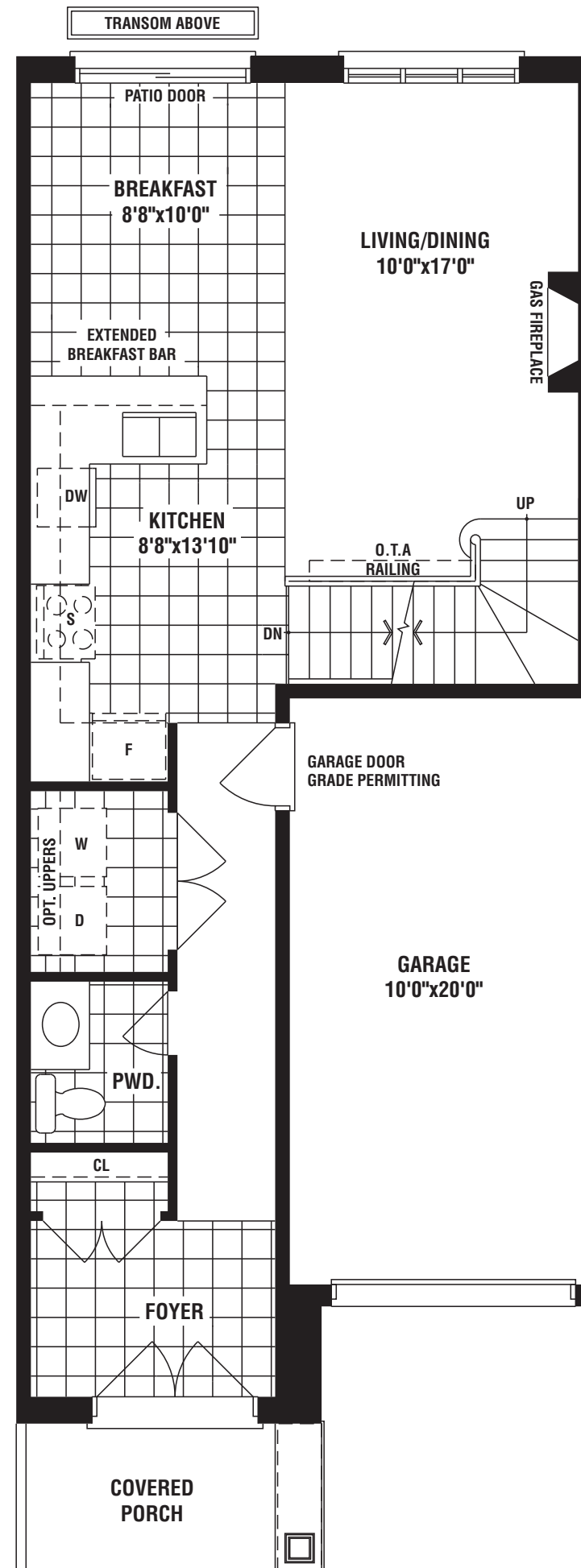
GROUND FLOOR PLAN EL. 'A'
