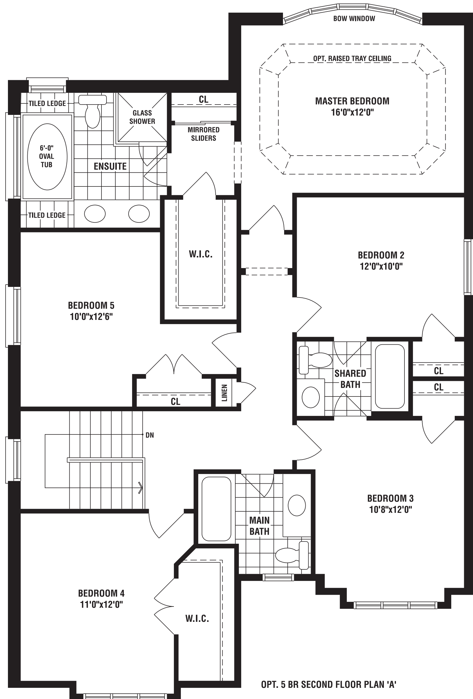
OPT. 5 BR SECOND FLOOR PLAN 'A'
